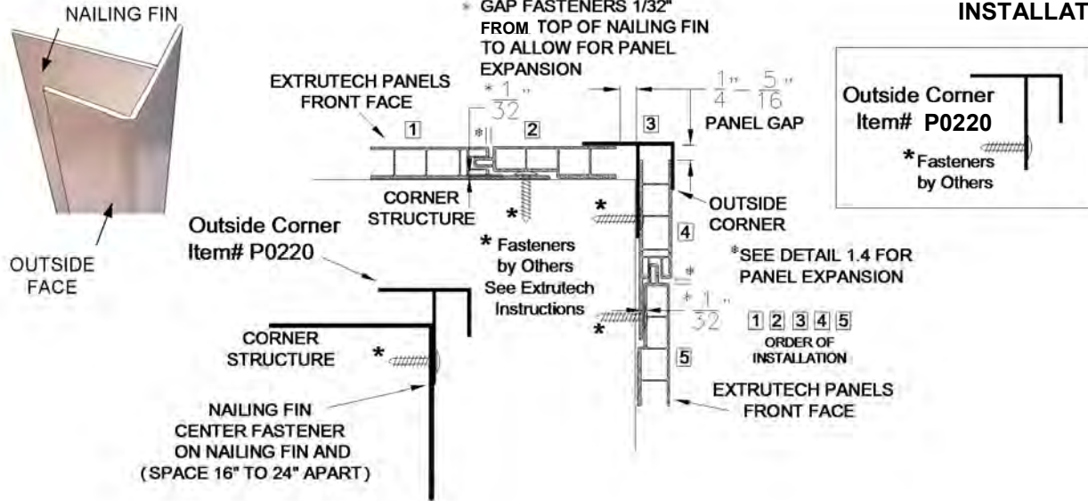
CORNER TRIM DETAIL 4.1-2 FOR VERTICAL PANEL INSTALLATION
