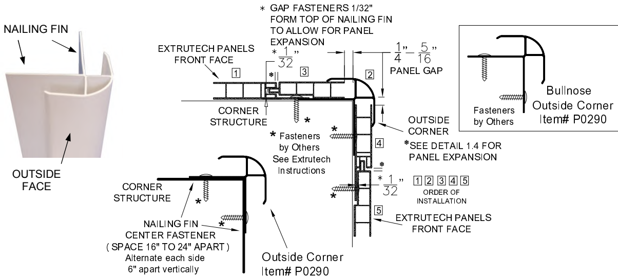
CORNER TRIM DETAIL 5.1-1 FOR VERTICAL PANEL INSTALLATION
