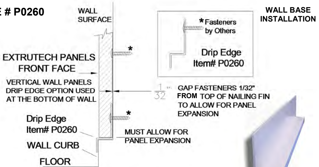
Drip-Edge Trim Cross Section FOR VERTICAL PANEL INSTALLATION FLOOR TRIM DETAIL 4.1-4
