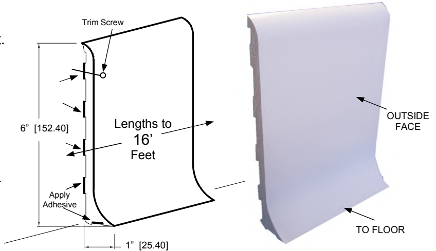
6" BASE BOARD DETAIL 6.00
