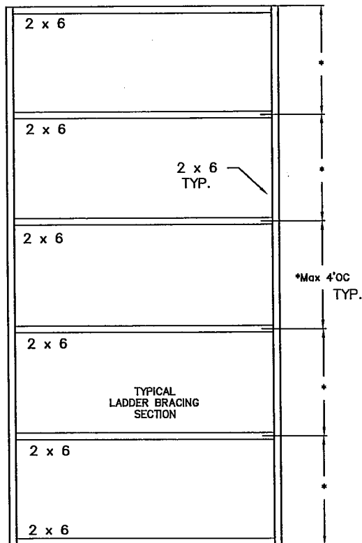
LADDER SHAPE BRACING
