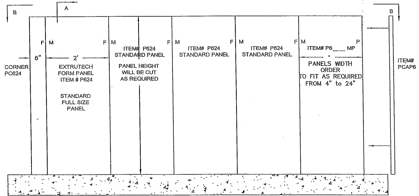
EXTRUTECH FORM PANELS (SIDE VIEW)
